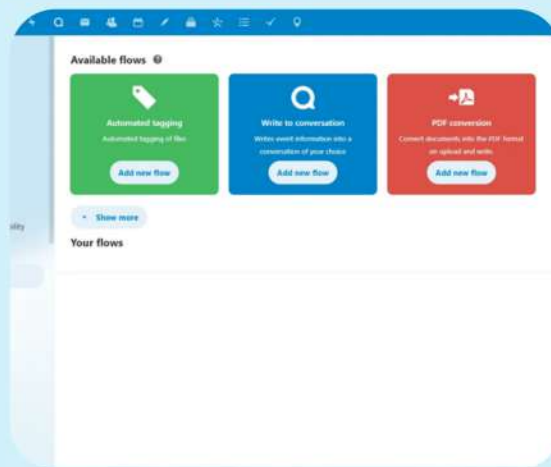
Workflow management
